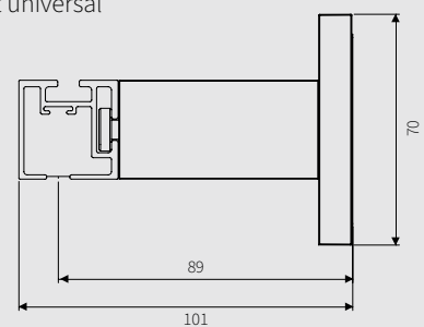
8,0 cm wall bracket universal
