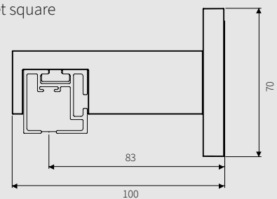
8,0 cm wall bracket square
