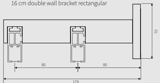
16 cm double wall bracket rectangular
