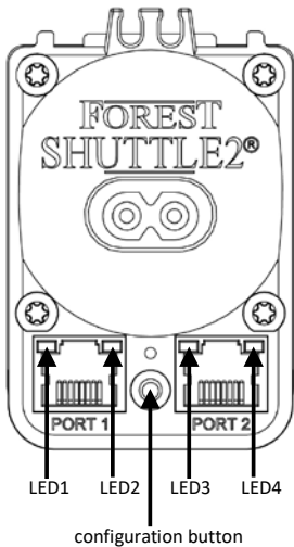
Bottom view of the Shuttle
