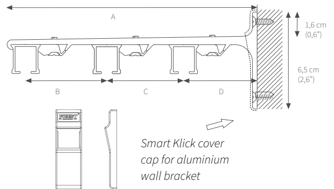
SK Aluminium Wall bracket triple
