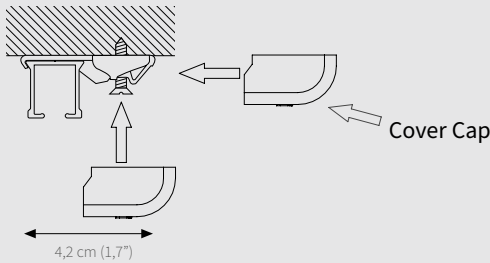
Smart Klick Ceiling bracket
