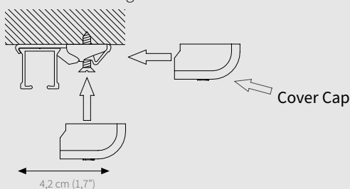
Smart Klick Ceiling bracket
