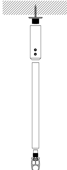
MTS Suspension Ceiling Bracket
