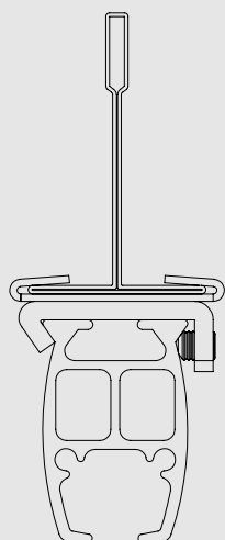
MTS Ceiling Bracket (for suspended ceiling)
